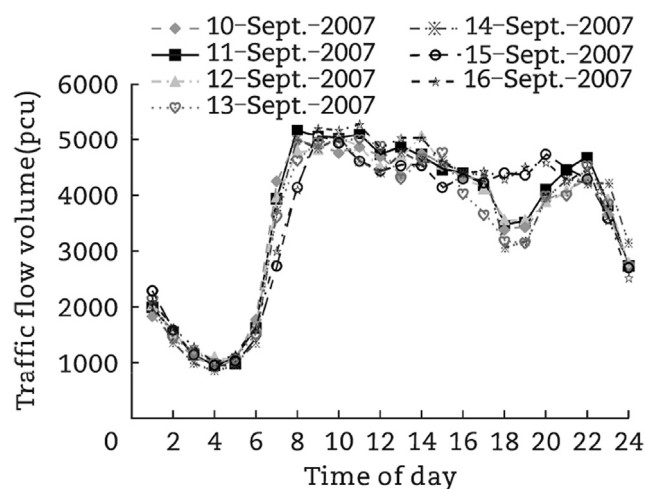
Fig. 3 – Weekly traffic flow volume in a detector location between Fuchengmen Interchange and Yuetanbei Interchange.
